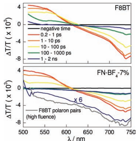
Figure 3. Transient absorption spectra of F8BT (top) and FN-BF 4 -7% (bottom) within 2 ns of excitation with integrated time regions indicated ( \lambda_{\text{exc}} = 490 \text{ nm} , fluence < 10^{14} photons/cm 2 ). The 1–2 ns spectrum is duplicated with a magnified scale in FN-BF 4 -7% for better comparison with early time spectra. Also shown (gray) is the spectrum of F8BT polaron pairs formed via exciton annihilation under significantly (>25-fold) higher fluence.
